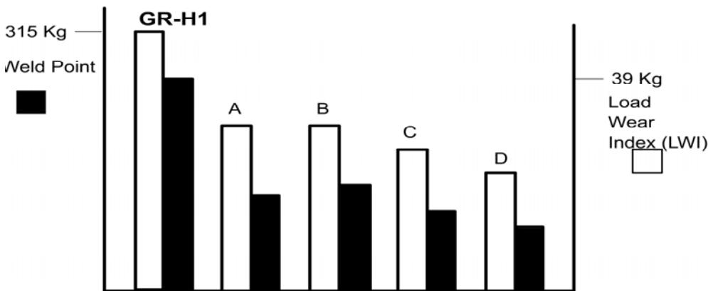
Dylon GR-H1 outperforms the competitors in the critical Four Ball Extreme Pressure Test
